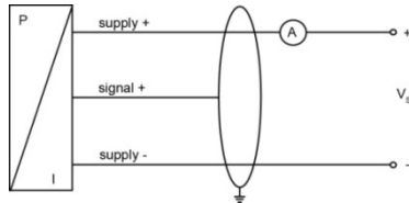
2-wire-system (current)
