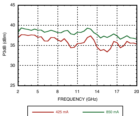
P3dB vs. Supply Current
