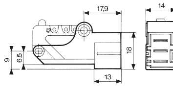
Housing 161J for connections W3 R5
